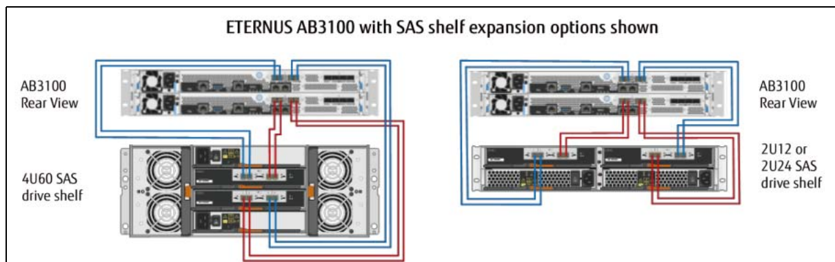
Figure 1 AB3100 with SAS expansion configuration
