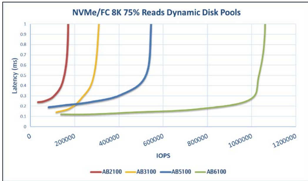
Figure 5 Performance results comparison for OLTP configuration
